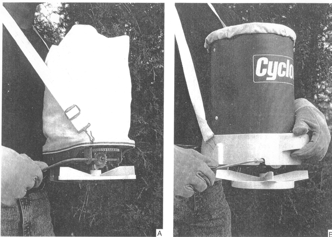
Figure 5.- (A) sack-type and (B) plastic hopper model of hand cranked spreaders.
